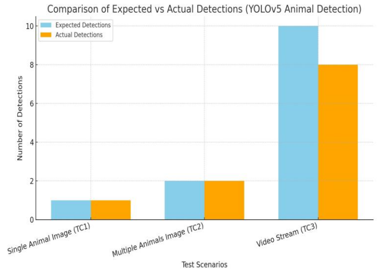
Fig. 4 graph comparing expected vs. actual detections for each test case in the YOLOv5-based Animal Intrusion Detection System
