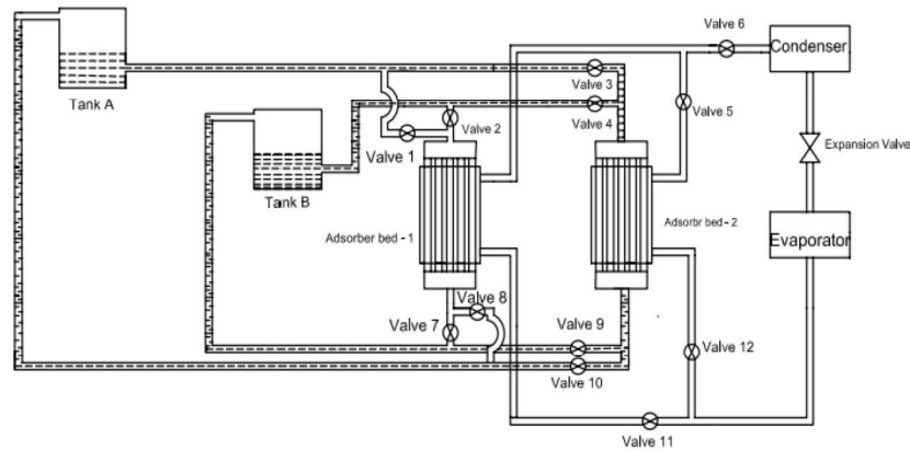
Figure 1. Working cycle of Vapour Adsorption Refrigeration
